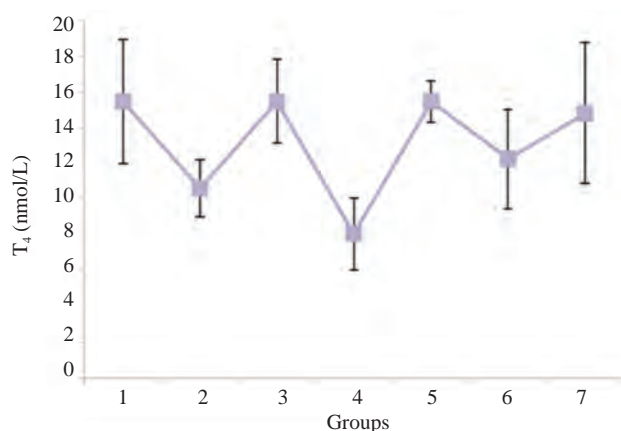
Figure 1. The concentrations of T 4 (nmol/L) in the control group and test groups.
