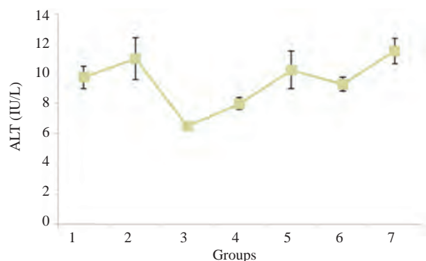
Figure 3. The concentration of ALT (IU/L) in the control group and test groups.
